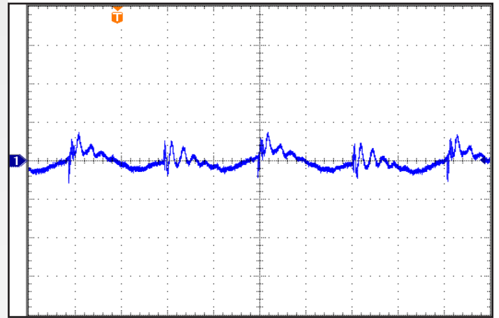
Figure 10: Output Voltage Ripple, V_{out} , at nominal input voltage and rated load current (50 mV/div). Load capacitance: 1 \mu F ceramic and 100 \mu F electrolytic capacitors. Bandwidth: 20 MHz. Timescale: 2.00 \mu s/div. See Figure 13.
