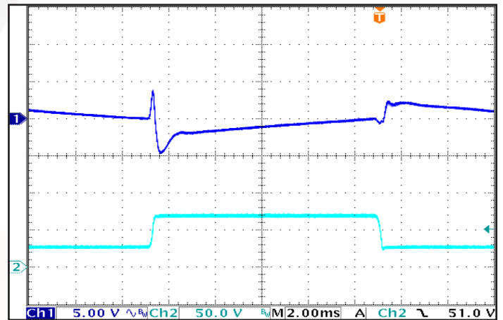
Figure 12: Output Voltage Response to Step-Change in Input Voltage, ( dV/dt = 250 V/ms). Load capacitance: 330 \mu F electrolytic output capacitance. Ch 1: V_{out} (5 V/div); Ch 2: V_{in} (50 V/div). Timescale: 2.00ms/div.
