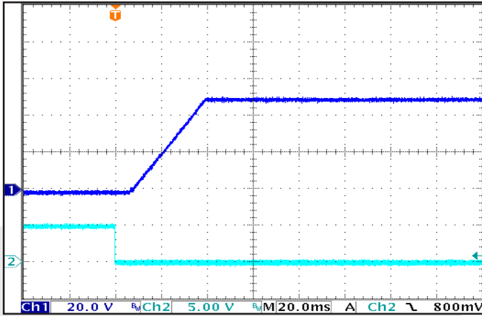
Figure 7: Typical Startup Waveform, input voltage pre-applied. Ch 1: V_{out} (20 V/div); Ch 2: ON/OFF Pin (5 V/div). Timescale: 20.0ms/div.
