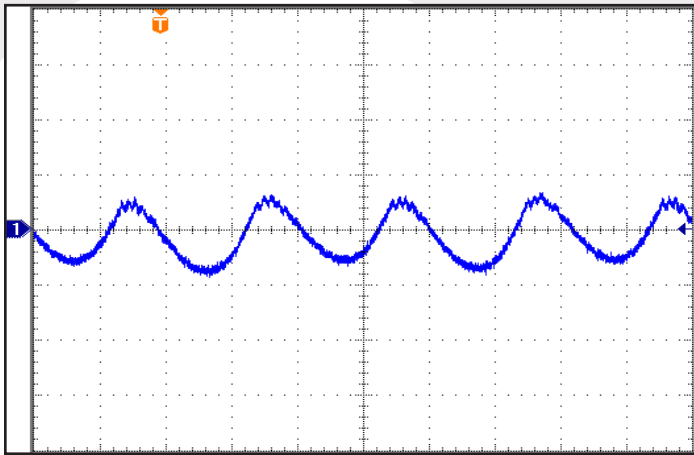
Figure 9: Input Terminal Current Ripple, i_C , at full rated output current and nominal input voltage with SynQor MCOTS filter module (1 A/div). Bandwidth: 20MHz. Timescale: 2.00 \mu s/div. See Figure 13.
